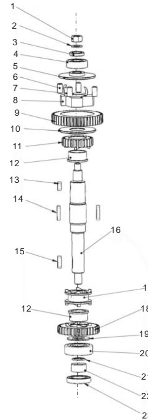
FIGURE 2 Centre axle
