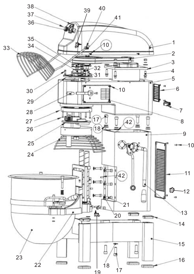
FIGURE 1 Mixer configuration
