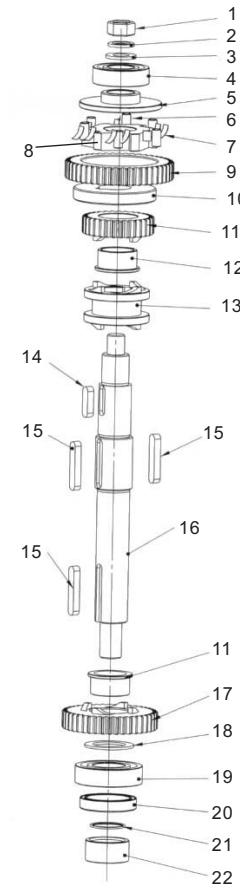
FIGURE 2 Centre axle
