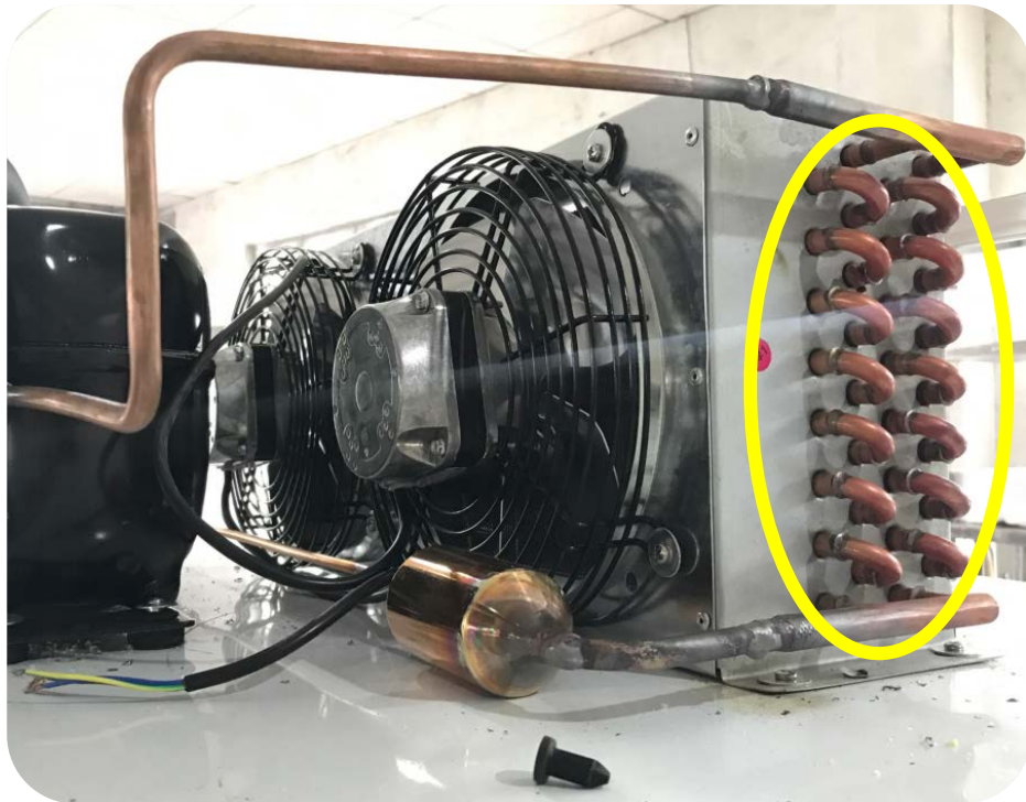
TT brand's condenser with more cooper pipes
