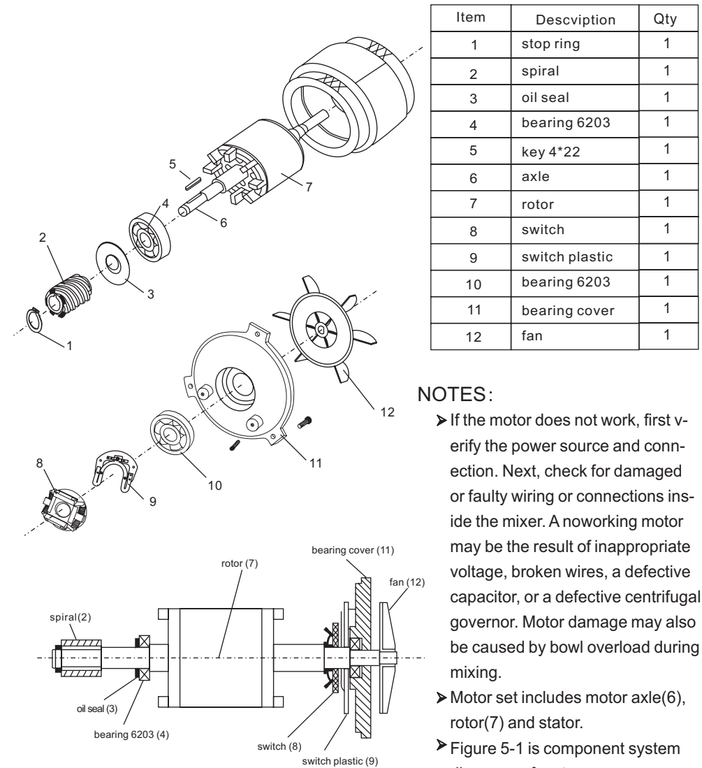
Figure 5 MOTOR UNIT
