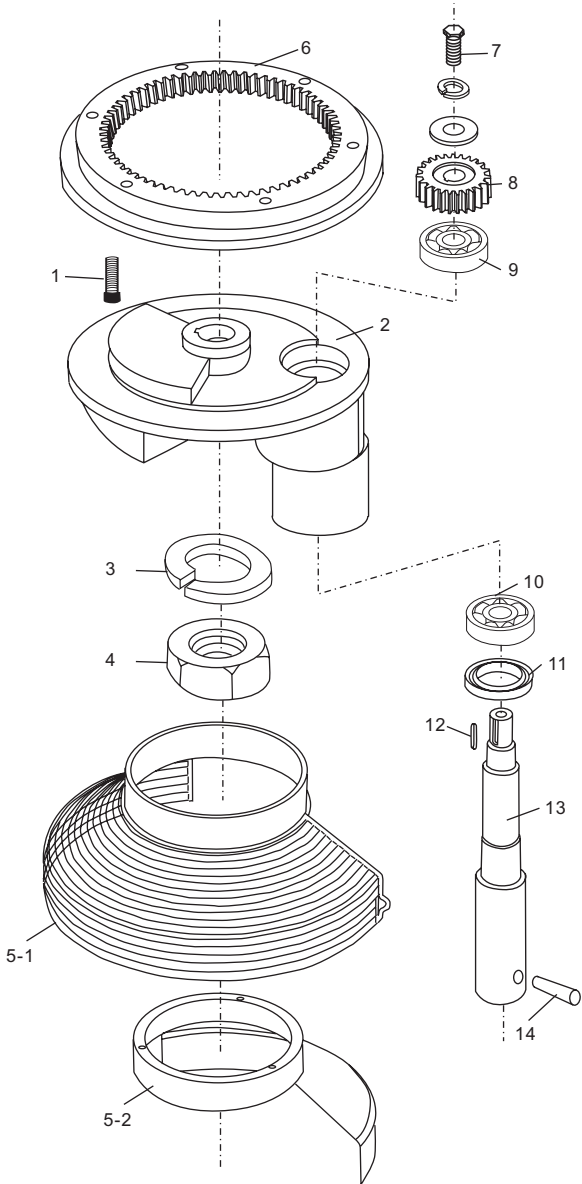
Figure 9 TURNING PLATE AND MIXING AXLE
