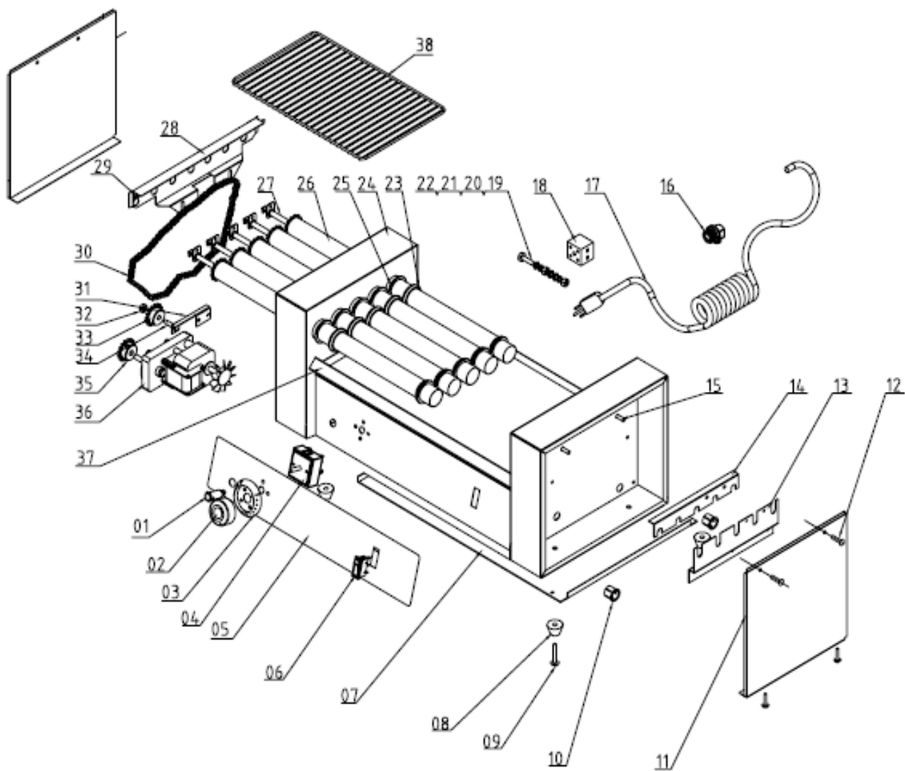
TT-R4 Electric hot-dog roller(5-roller)
