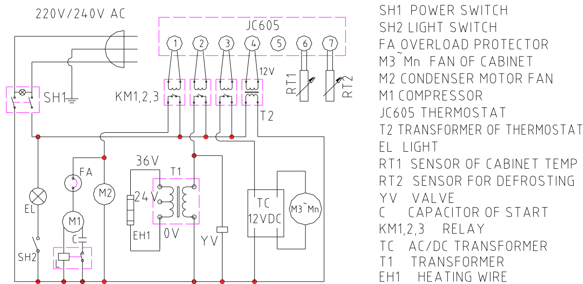
Electric Wiring Diagram
